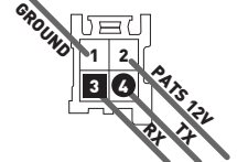
CONNECTOR C - GREEN FOUND 8 INCHES LOWER ON PATS HARNESS
