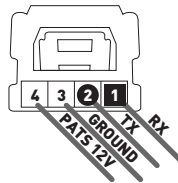
CONNECTOR D - WHITE LOCATED AT IMMOBILIZER NEAR KEY BARREL
