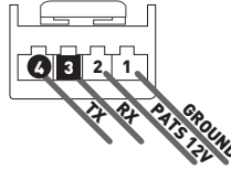
CONNECTOR D - WHITE LOCATED AT IMMOBILIZER NEAR KEY BARREL
