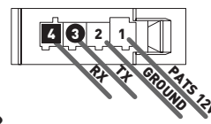
CONNECTOR B - GREEN LOCATED AT IMMOBILIZER NEAR KEY BARREL
