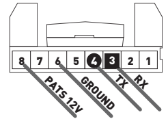
CONNECTOR F - WHITE LOCATED AT IMMOBILIZER NEAR KEY BARREL
