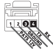
CONNECTOR E - BLACK LOCATED AT IMMOBILIZER NEAR KEY BARREL
